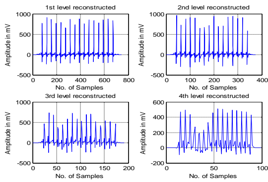
Fig. 9: Reconstructed Signal
