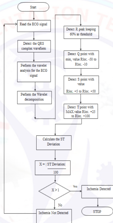
Fig. 6: Flowchart for the Detection of Ischemia
