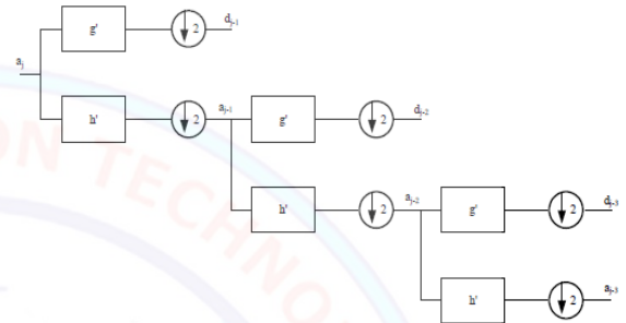
Fig. 4: Wavelet Decomposition [6]
