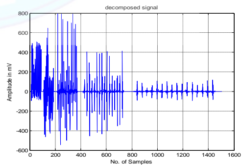
Fig. 8: Decomposed Signal
