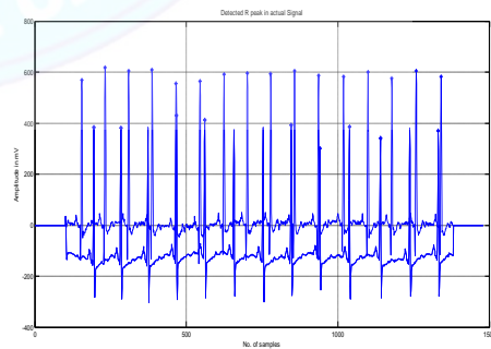
Fig. 16: Detected R Peak in Actual Signal
