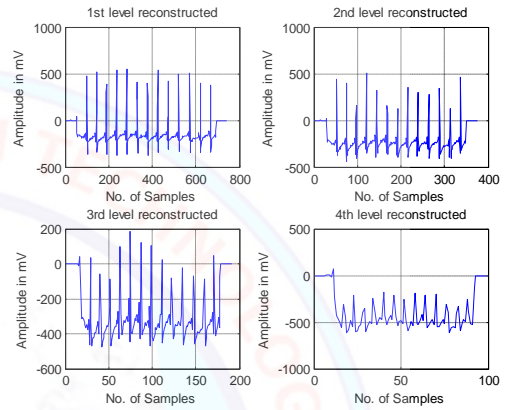
Fig. 14: Reconstructed Signal
