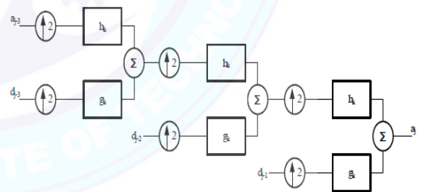
Fig. 5: Wavelet Reconstruction[6]
